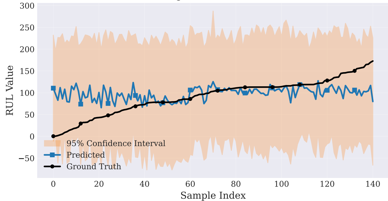
Remaining Useful Life (Validation)
