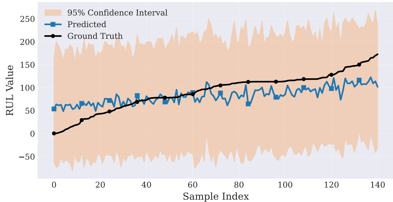
Remaining Useful Life (Validation)
