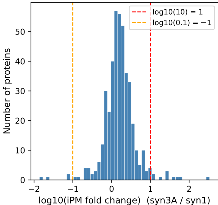
Protein log10 fold change distribution
