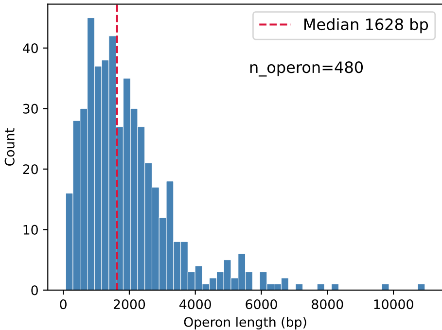
Operon length distribution
