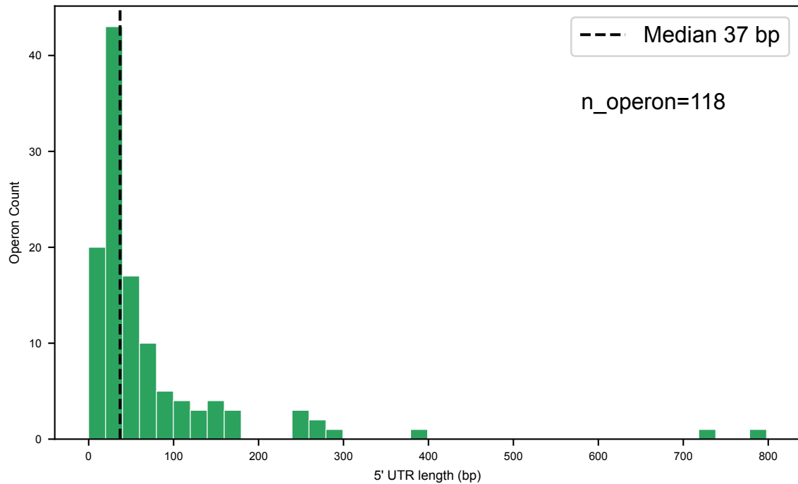
5' UTR (TSS → first sense gene 5' end)
