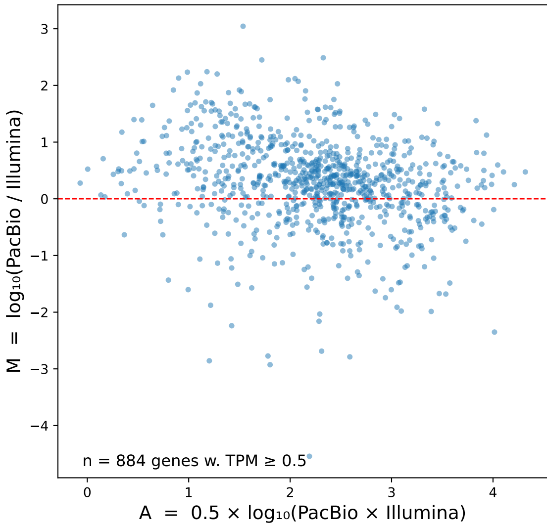
MA Plot: PacBio vs Illumina sense TPM
