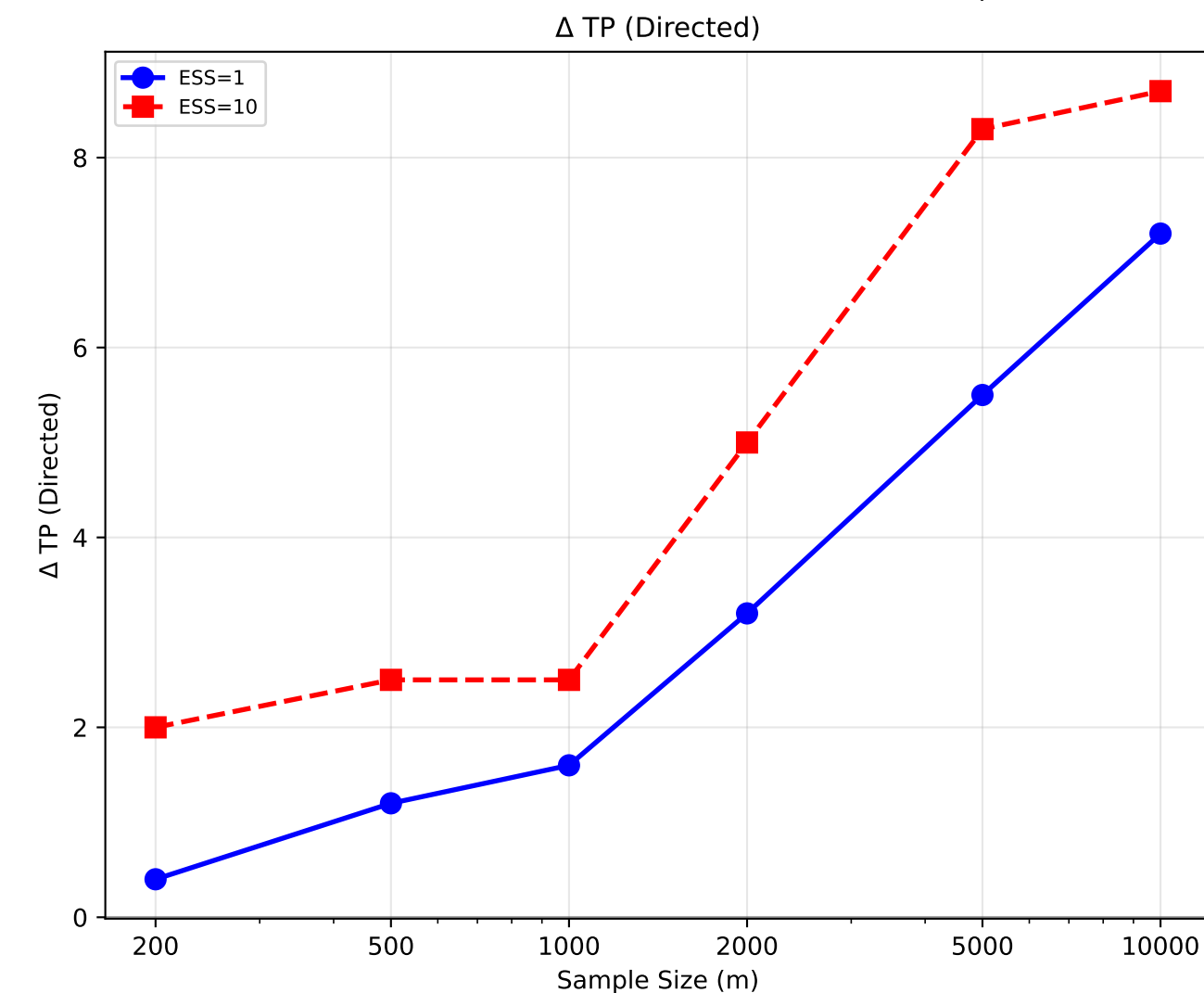
Contrast 1: HC_BDeu vs hierarchy (Value of hierarchical constraint)
