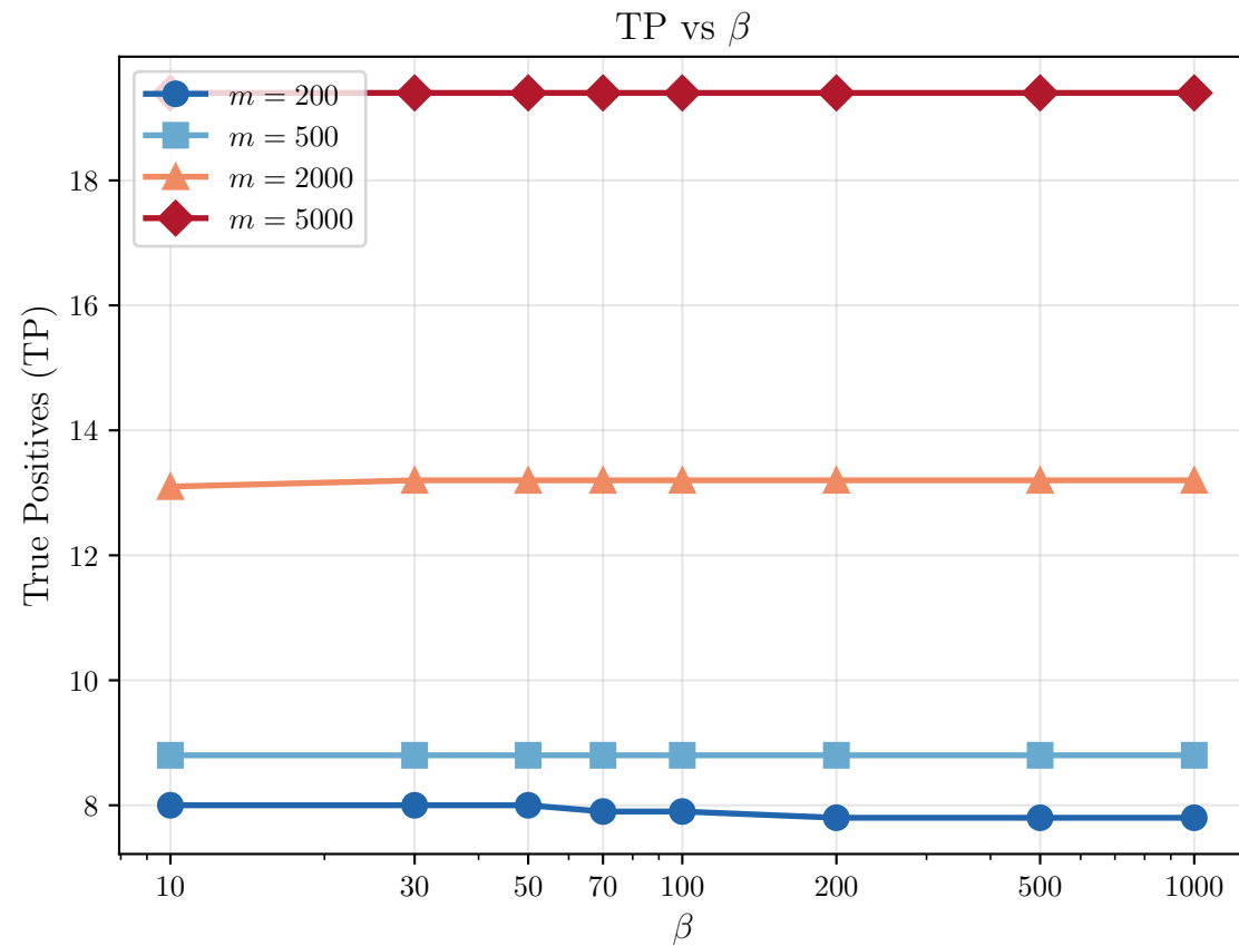
Sensitivity to \beta (hierarchy_mono_score, \alpha = 0.9 , ESS=10)
