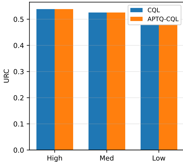
Uncertainty--Return Correlation
