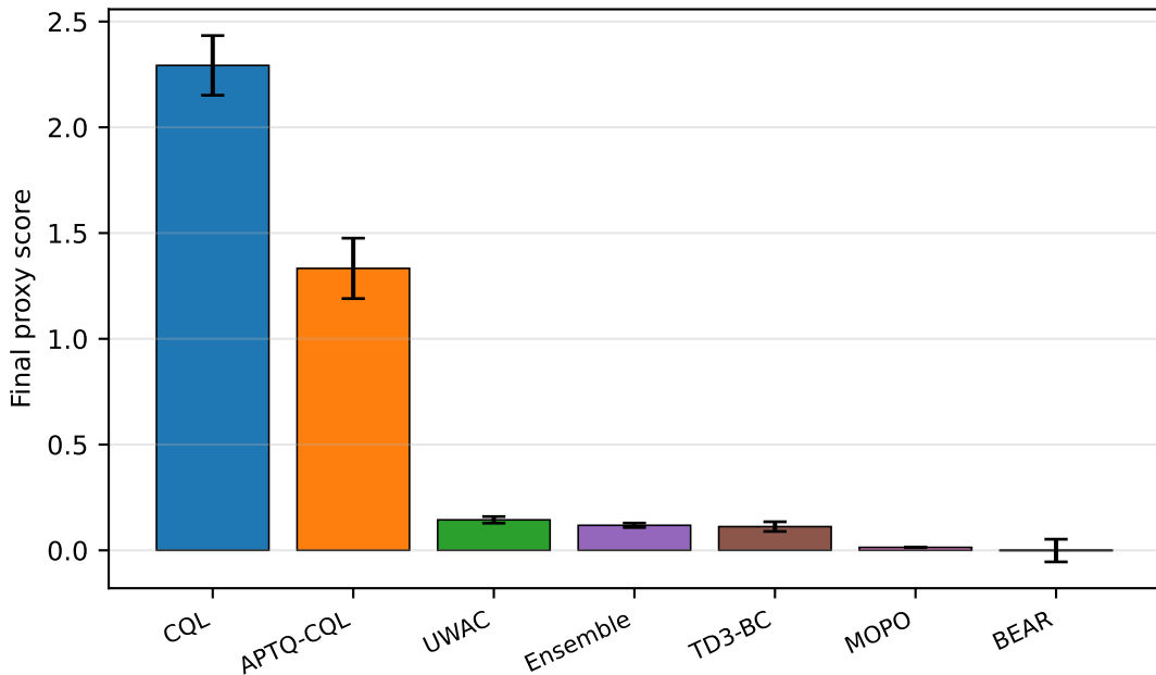
Final score (mean of last 3 checkpoints, 3 seeds)
