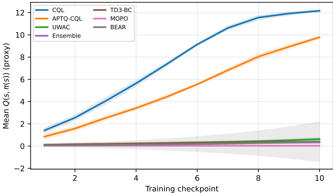
Unified offline policy-value proxy during training
