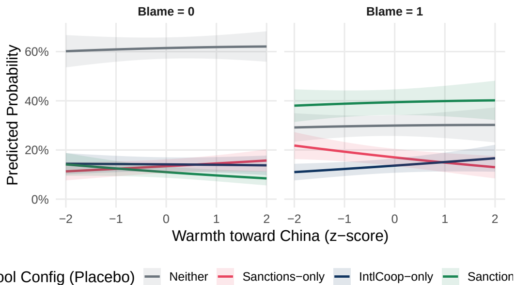
Figure A1: Placebo test: Interaction plot for sanctions \times international cooperation composite as dependent variable. The placebo pairing shows a comparable blame-driven shift ( \Delta = 0.327 ), indicating that the S+A effect is not fully specific to fentanyl cooperation.
