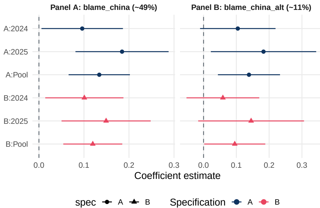
Figure A2: Coefficient forest plot for the warmth × blame interaction across model specifications. Point estimates with 95% confidence intervals.
