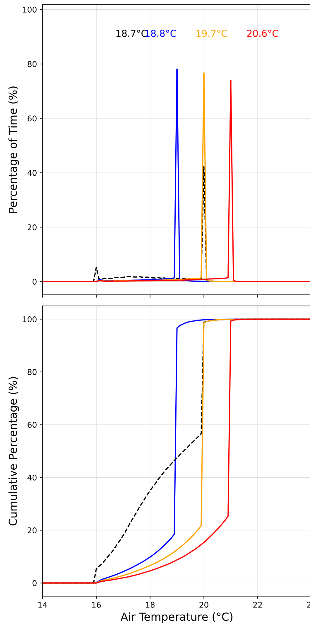
Heating Hours 6-8 + 12-14 + 18-23
