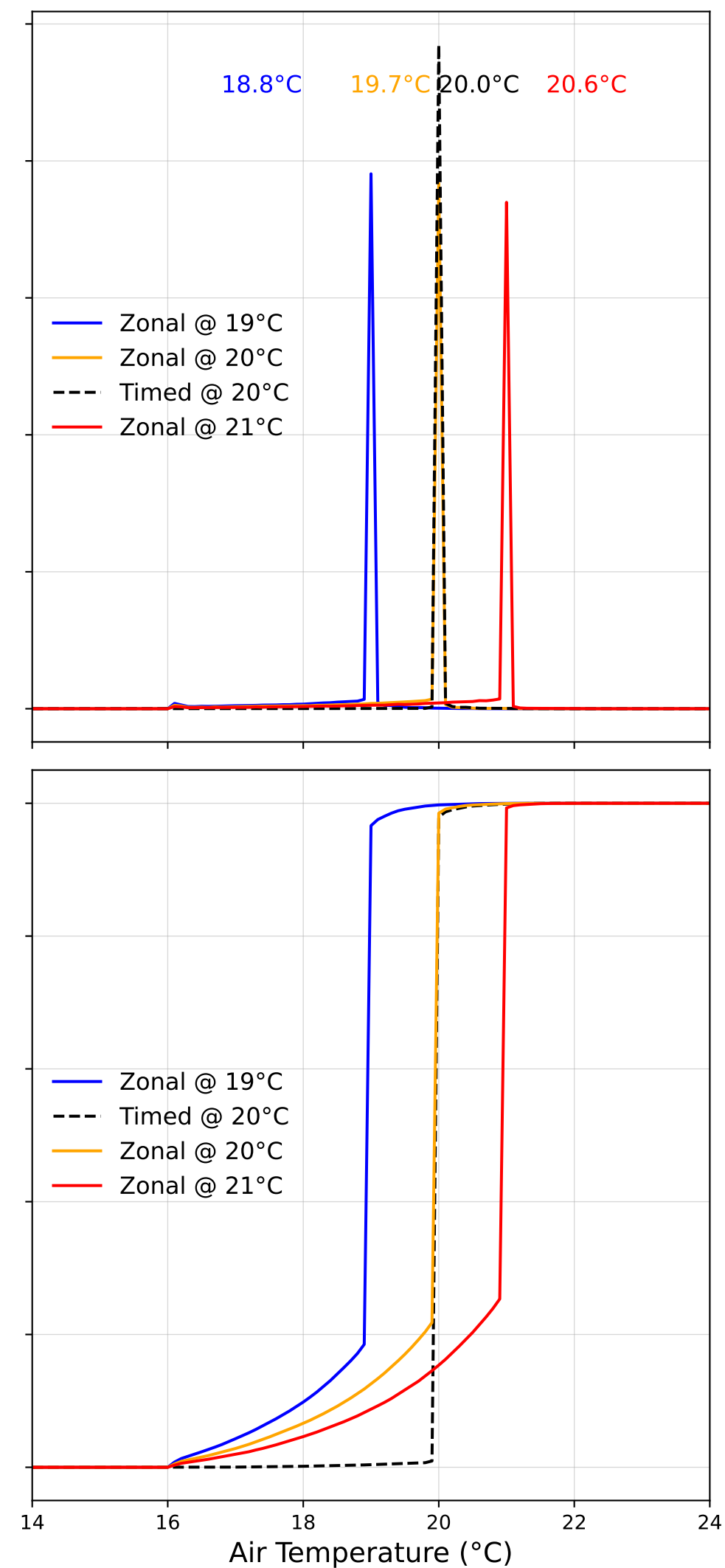
Heating Hours 6-23
