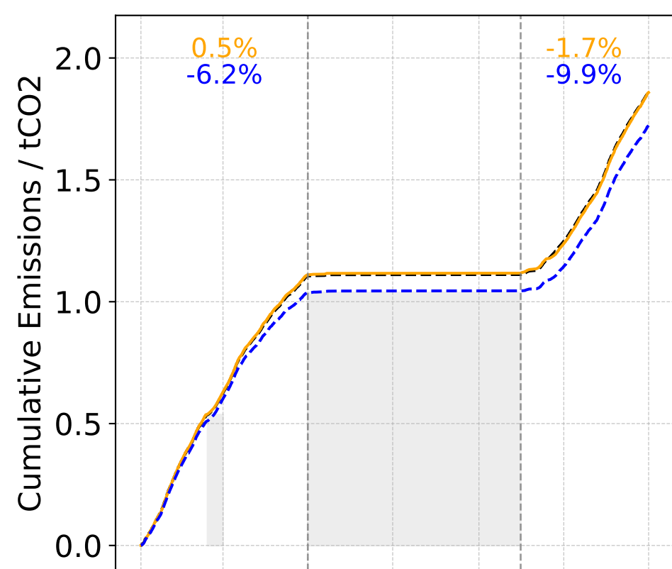
Heating Hours 6-8 + 12-14 + 18-23
