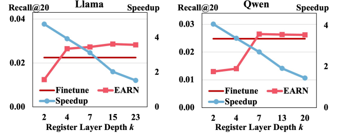
Figure 6: Effect of register layer depth k .
