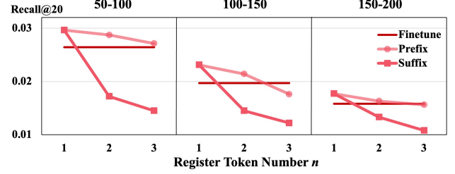
Figure 8: Effect of register token number n under different prompt length.
