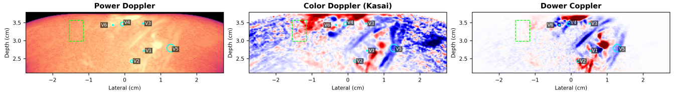
Figure 4: Regions used for the CNR and gCNR measurements in fig. 5. Cyan circles indicate the largest circular signal ROIs fully contained inside the six exported vessel masks. The dashed green rectangle is the shared background ROI used for every vessel and every Doppler display.
