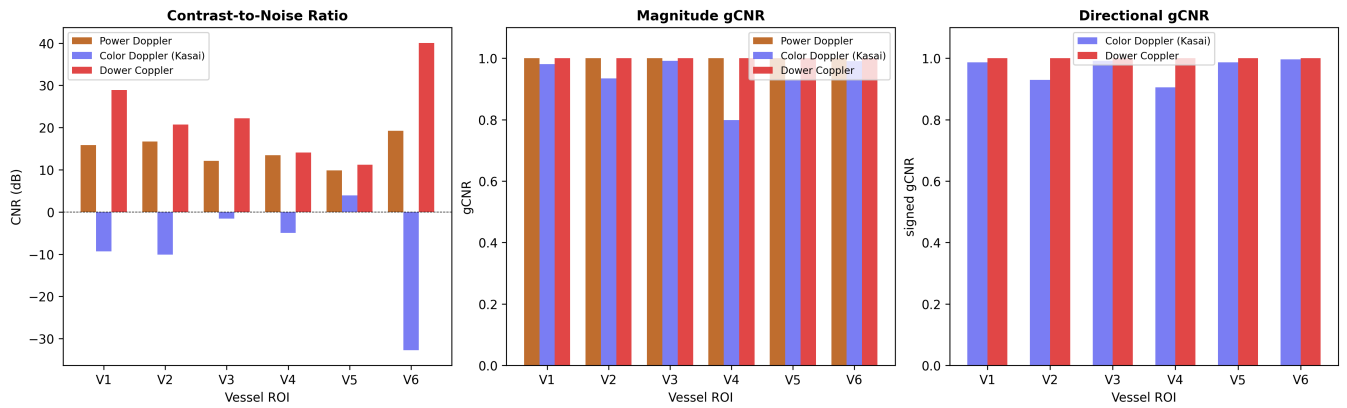
Figure 5: Left: CNR in dB across six vessel ROIs. Dower Coppler has median CNR 21.5 dB across the six selections (range 11.2–40.1 dB), exceeding both power Doppler and Kasai color Doppler in all ROIs. Middle: magnitude generalized CNR ( 1 - \text{histogram overlap} ) using power Doppler, |\text{color Doppler}| , and |\text{Dower Coppler}| . Right: directional gCNR computed on the signed color Doppler and signed Dower Coppler values; power Doppler is omitted because it has no direction sign.
