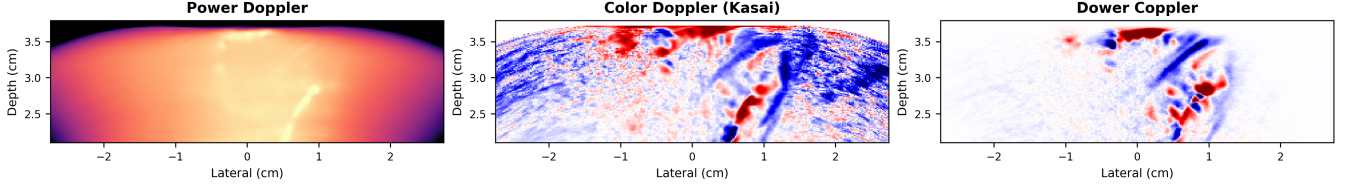
Figure 1: Intact-skull transcranial human cortex imaging from a 3D matrix-array acquisition (median of 480 Doppler buffers, plane-wave compounding). This panel shows a central reconstructed elevation plane from the lateral-elevation-depth Doppler volume. Left: power Doppler, displayed with a robust positive-pixel dB window, shows vessel structure but no directional information. Center: Kasai color Doppler ( \angle R_1 ) reveals direction but is dominated by noise. Right: Dower Coppler ( v_\phi G_R R^2 , K = 5 ) combines multi-lag coherence weighting with directional information from the phase slope and fit quality. Opposing flow directions in adjacent cortical vessels are resolved in this intact-skull human transcranial acquisition.
