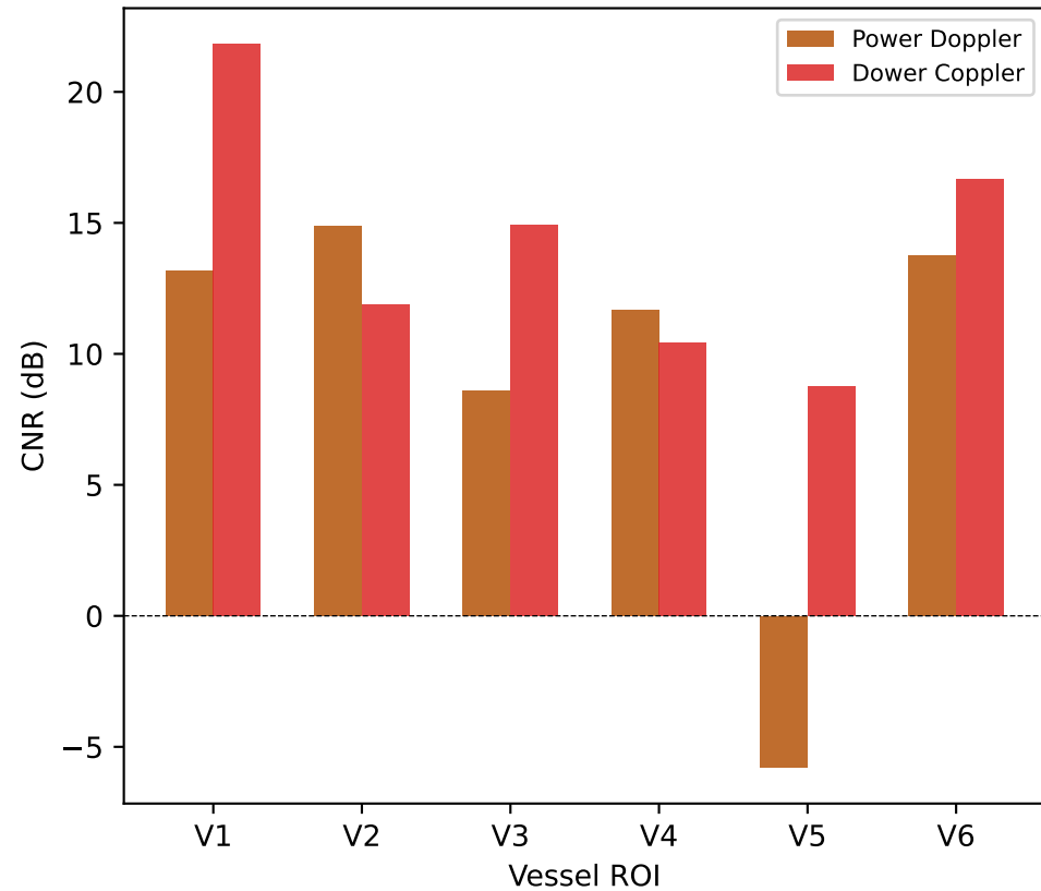
Contrast-to-Noise Ratio
