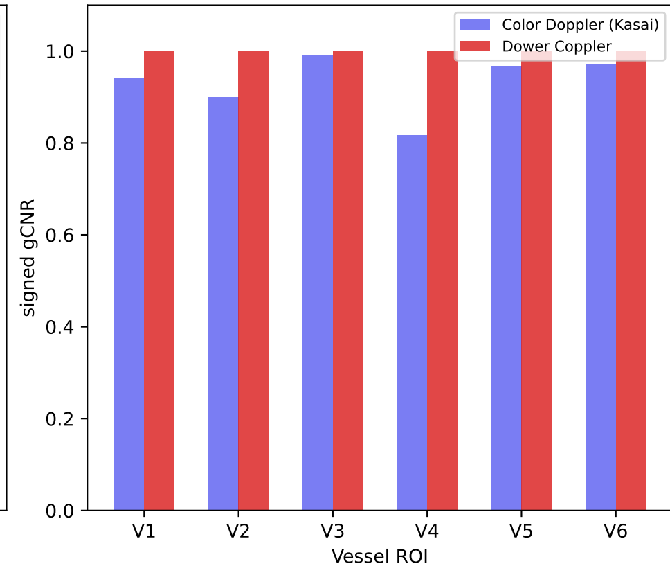
Directional gCNR
