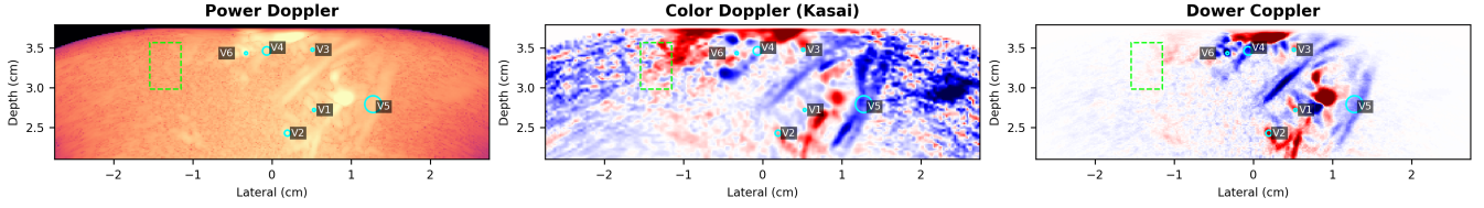
Figure 3: Regions used for the CNR and gCNR measurements in fig. 4. Cyan circles indicate the largest circular signal ROIs fully contained inside the six exported vessel masks. The dashed green rectangle is the shared background ROI used for every vessel and every Doppler display.
