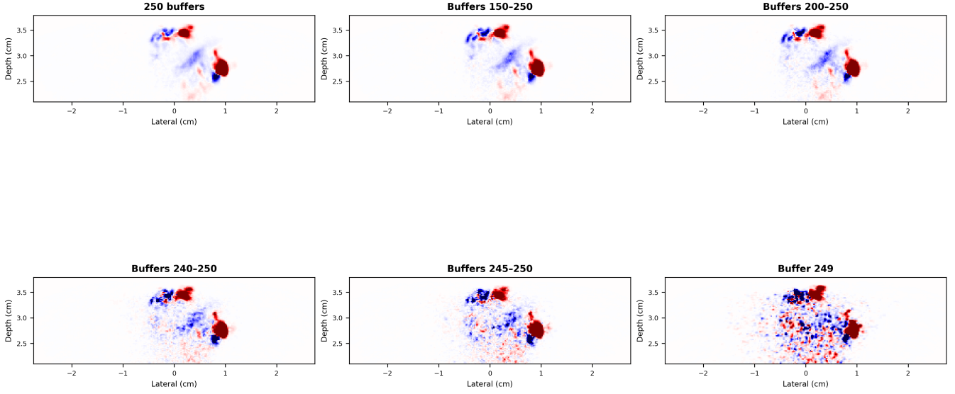
Figure 5: Dower Coppler maps computed from different numbers of Doppler buffers (same color scale throughout). The vessel pattern and flow direction assignment are stable from 250 buffers down to 5 buffers. At a single buffer, the major vessels remain identifiable but background noise increases.
