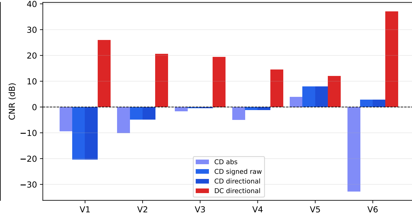
Histogram separability alternatives
