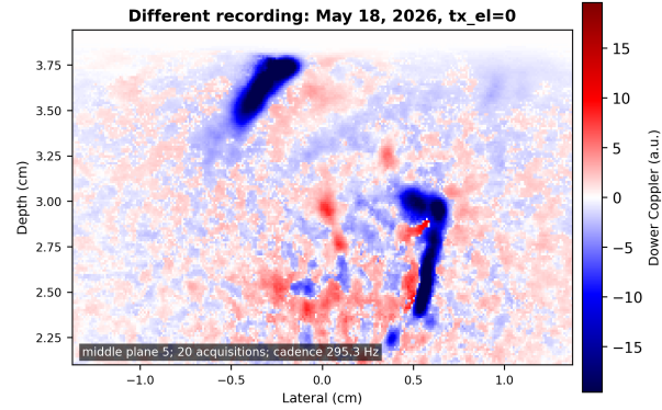
Figure A4: Qualitative check from a different May 18, 2026 recording using 20 acquisitions, compounded-frame cadence 295.3 Hz, f_0 = 2.75 MHz, c = 1600 m/s, SVD cutoff 0.08, and K = 5 .
