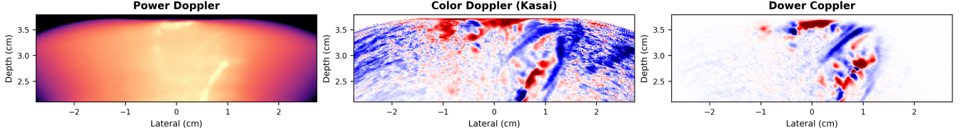
Figure 1: Intact-skull transcranial cortex imaging from a 3D matrix-array acquisition (median of 480 Doppler buffers, plane-wave compounding), shown on a central reconstructed elevation plane. Left: power Doppler, displayed with a robust positive-pixel dB window, shows vessel structure but no directional information. Center: Kasai color Doppler ( \angle R_1 ) reveals direction but is dominated by noise. Right: Dower Coppler ( v_\phi G_R R^2 , K = 5 ) combines multi-lag coherence weighting with directional information from the phase slope and fit quality. Opposing flow directions in adjacent cortical vessels are clearly resolved.
