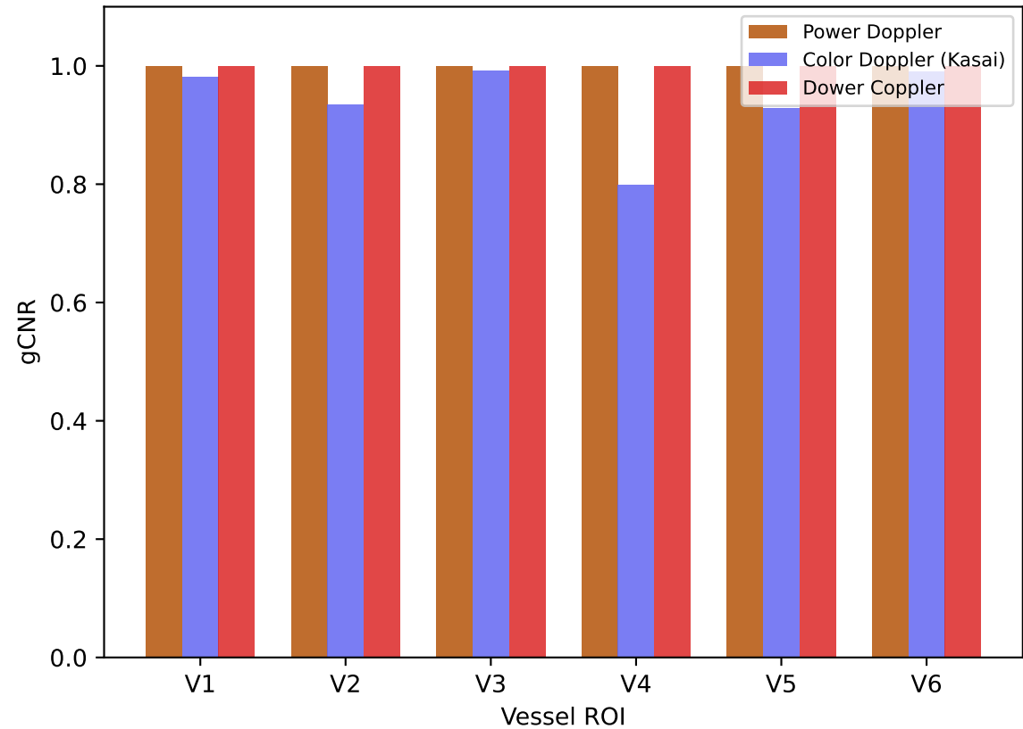
Generalized CNR
