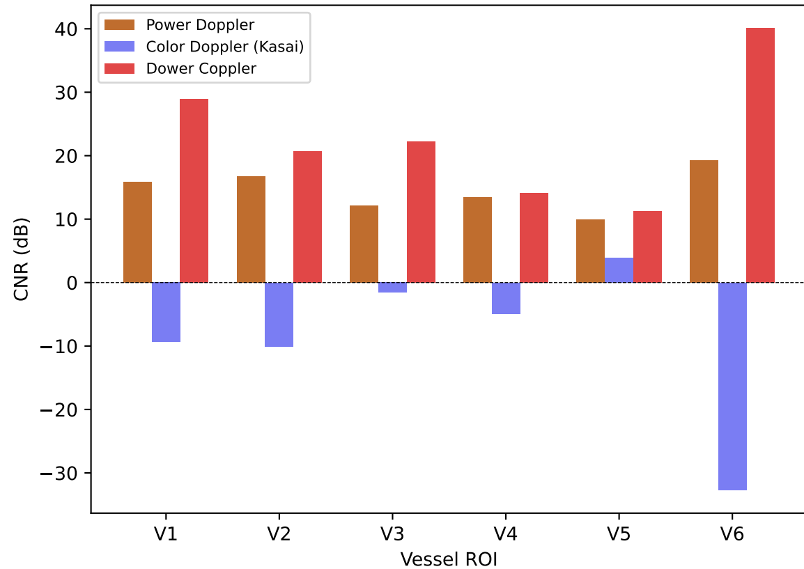
Contrast-to-Noise Ratio
