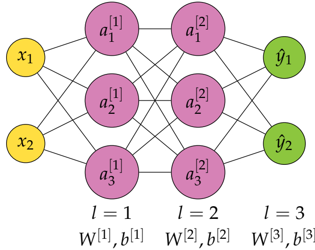
Figure 19.9: A visualization of a neural network with layers of 2, 3, 3, and 2
