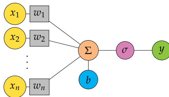
Figure 19.2: Visualization of a single neuron
