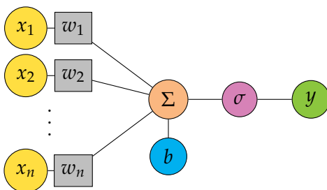
Figure 20.2: Visualization of a single neuron
