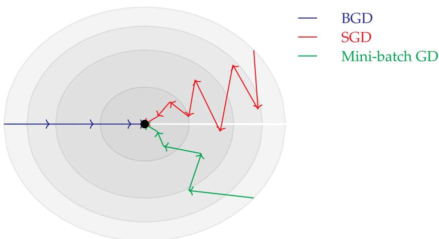
Figure 20.7: Visualization of Different Types of Gradient Descent
