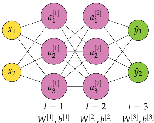
Figure 20.9: A visualization of a neural network with layers of 2, 3, 3, and 2
