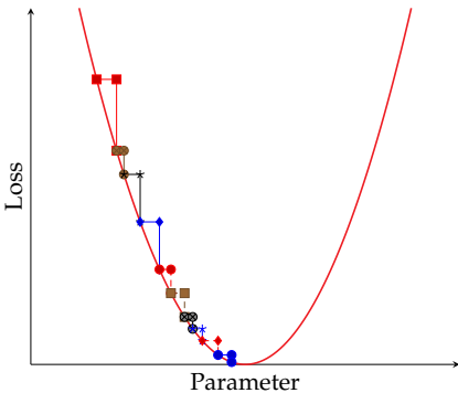
Figure 20.6: Visualization of Case II
