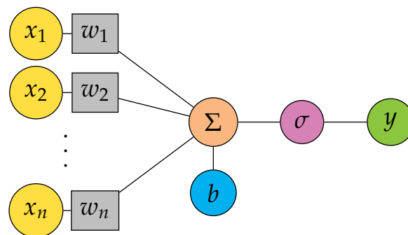
Figure 15.2: Visualization of a single neuron
