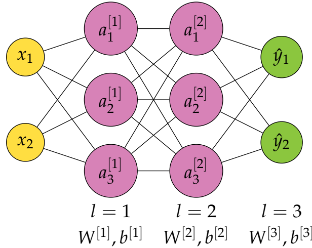
Figure 15.9: A visualization of a neural network with layers of 2, 3, 3, and 2
