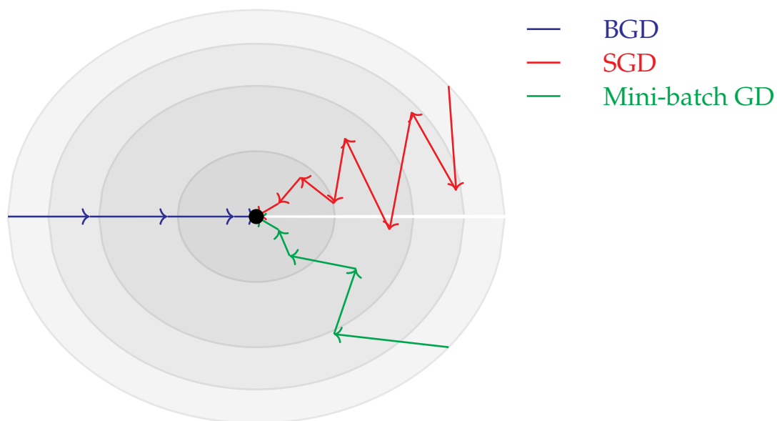
Figure 17.7: Visualization of Different Types of Gradient Descent
