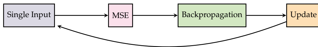
Figure 17.10: Overview of the Simple Learning Engine
