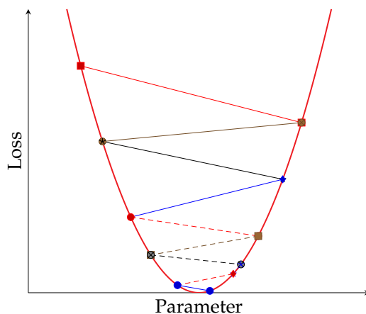
Figure 16.5: Visualization of Case I
