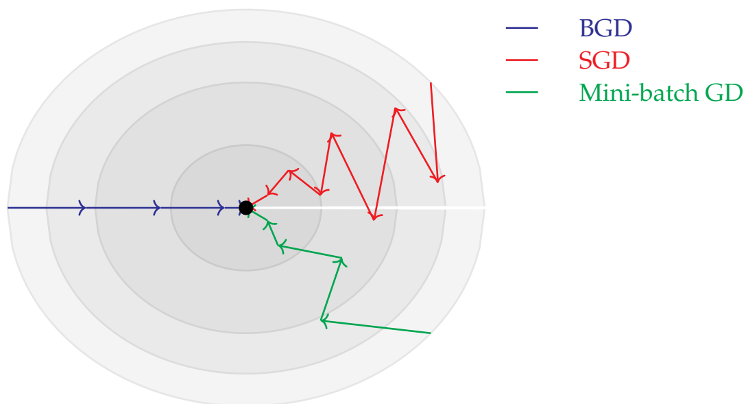
Figure 16.7: Visualization of Different Types of Gradient Descent
