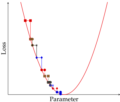
Figure 19.6: Visualization of Case II
