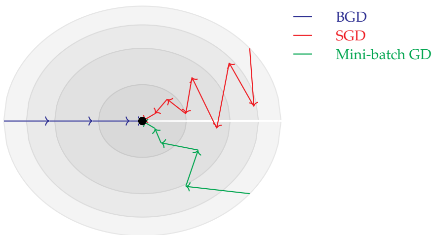
Figure 19.7: Visualization of Different Types of Gradient Descent
