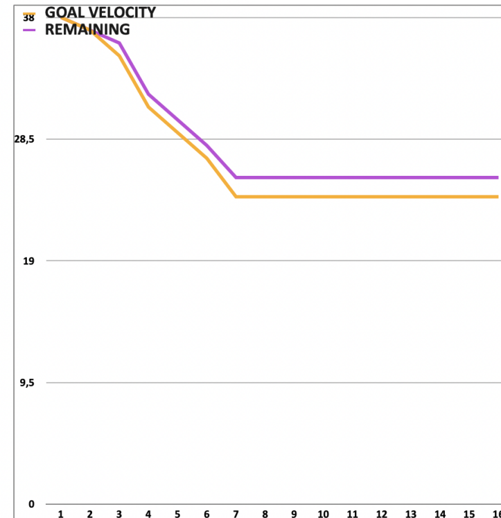
BURNDOWN
