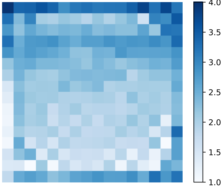
Mean depth ( \mu=2.25 )
