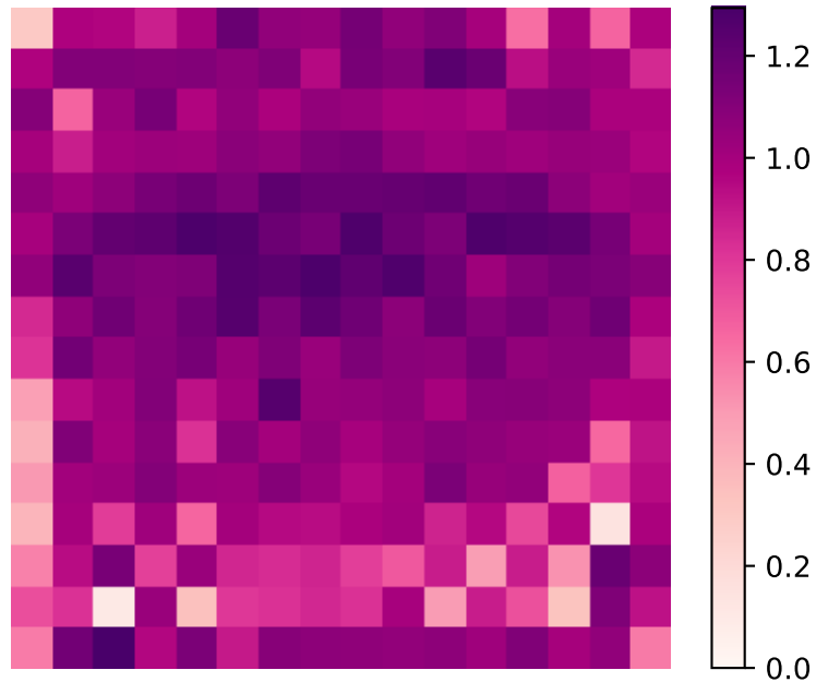
Per-position std (mean=1.000)
