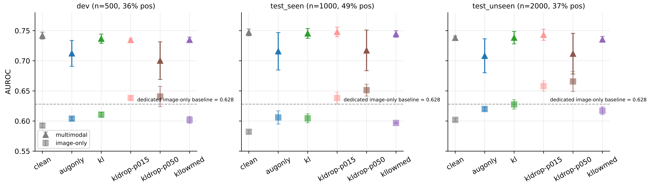
Image-branch revival: multimodal (▲) and image-only (■) forward AUROC per recipe
