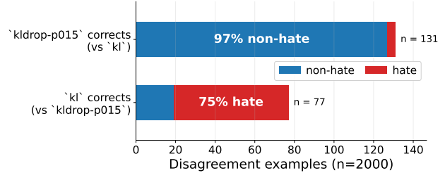
Figure 2. Per-example disagreements between KLDrop-p015 and KL on test_unseen ( n=2000 ), split by gold label.
