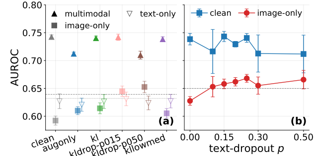
Figure 1. (a) Per-branch forward AUROC (mean over 3 splits \times 3 seeds). (b) Dropout sweep ( test_unseen ).
