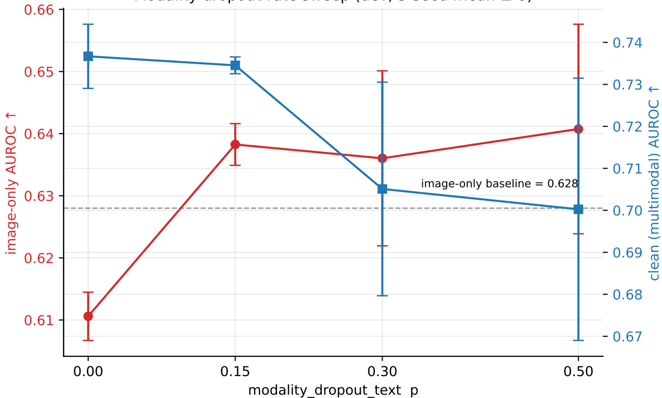
Modality-dropout-rate sweep (dev, 3-seed mean \pm \sigma )
