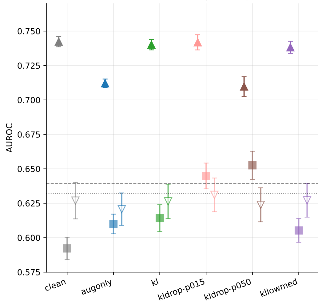
(a) Per-branch AUROC, split-averaged
