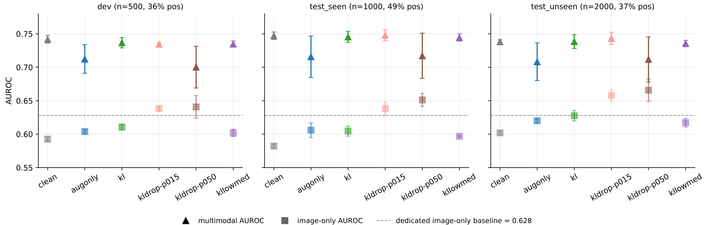
Image-branch revival: multimodal (▲) and image-only (■) forward AUROC per recipe
