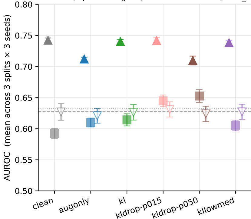
Per-branch forward AUROC, split-averaged (bar = \sigma across dev / test_seen / test_unseen)
