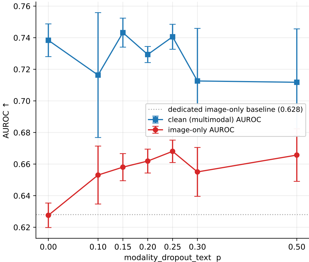
Modality-dropout-rate sweep (test_unseen, 3-seed mean \pm \sigma )
