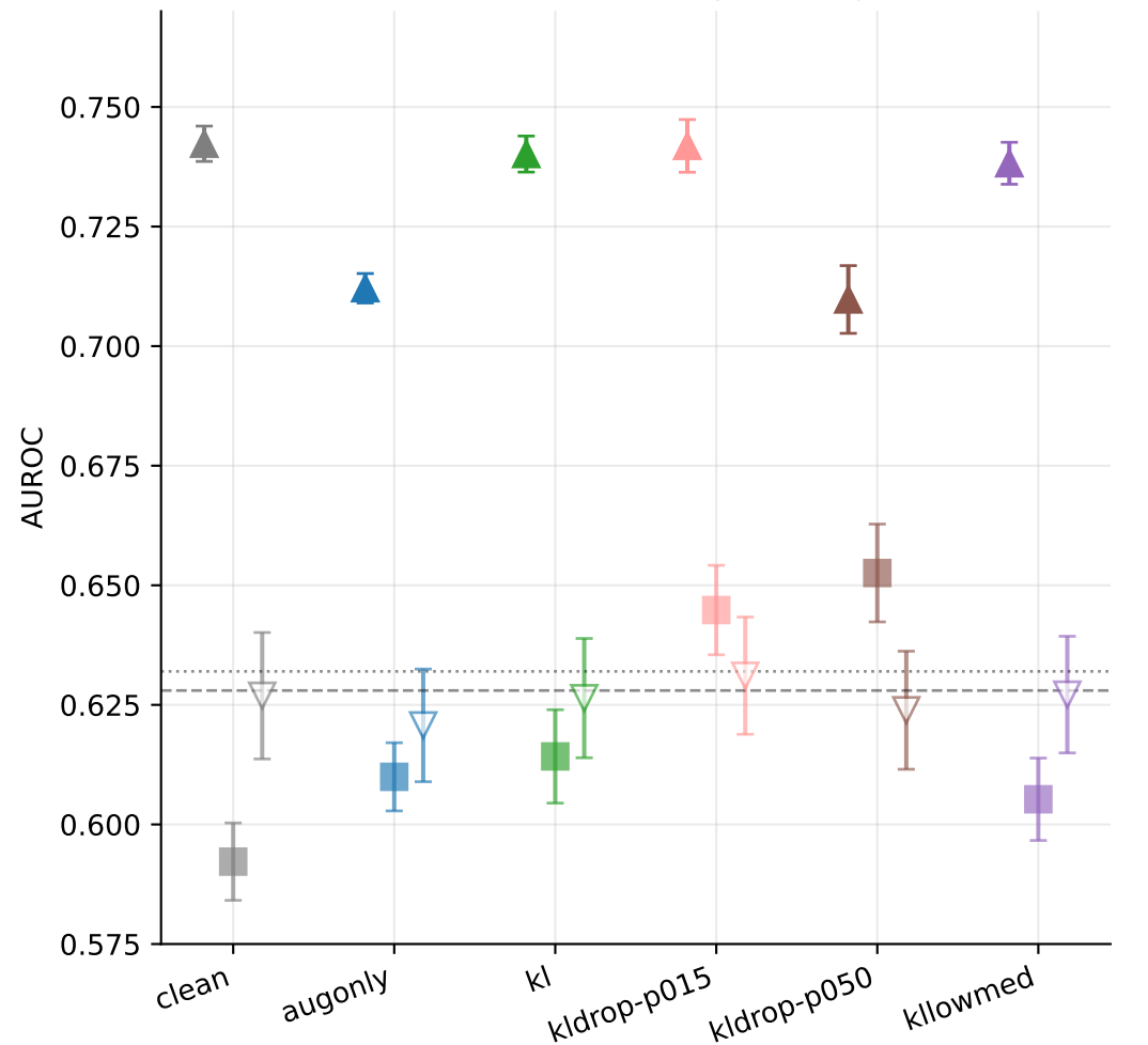
(a) Per-branch AUROC, split-averaged
