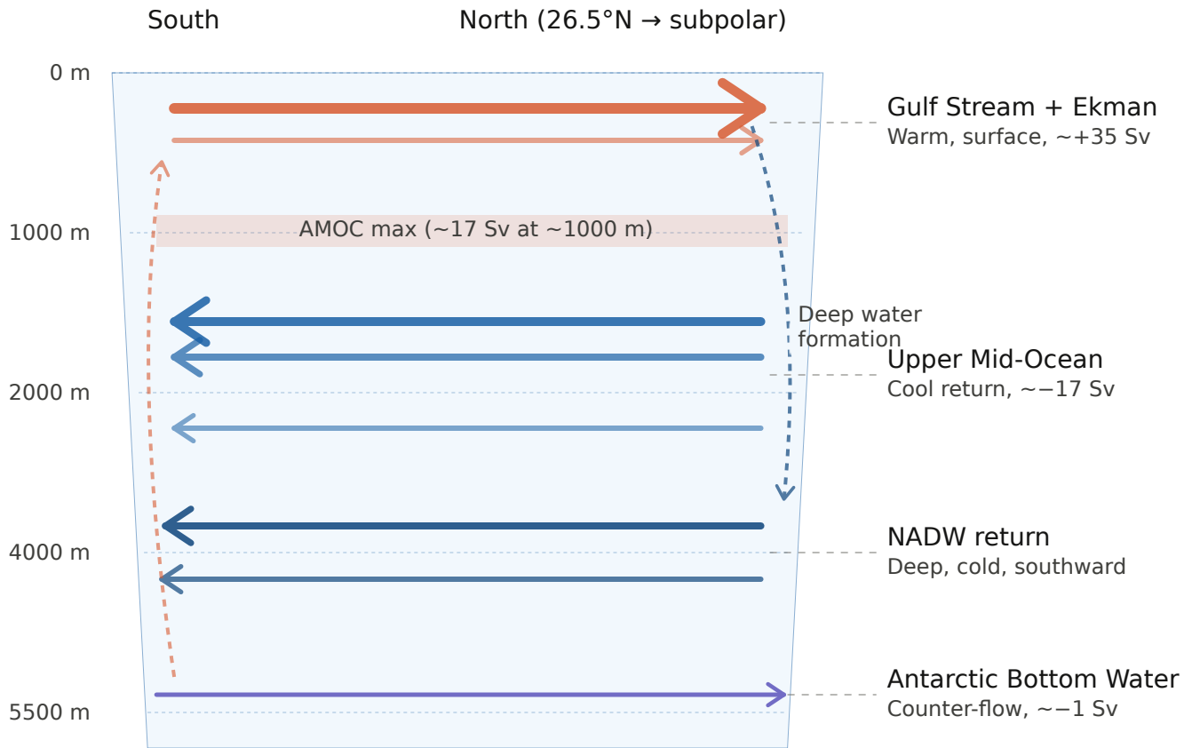
Schematic vertical slice of the Atlantic at RAPID latitude (26.5°N) and northward Arrow thickness \approx transport magnitude · colour = water temperature
