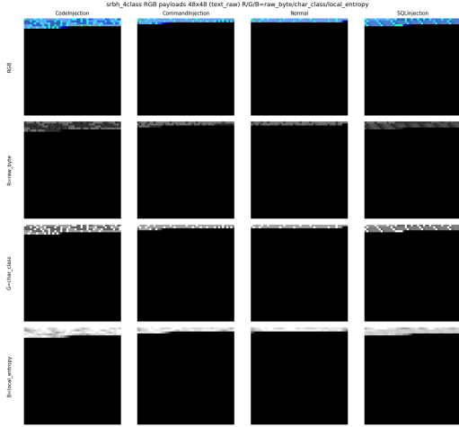
Fig. 1. Byte images of SR-BH 2020 requests (URI and body, 48×48, RGB). Most requests are short (median 96 bytes) and fill only the top few rows (median two).
