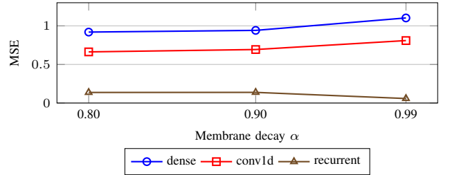
Figure 5. MSE vs. membrane decay \alpha for SNN modes (direct encoding, V_{th} = 1.0 ). For the recurrent mode, \alpha = 0.99 more than halves MSE ( 0.137 \rightarrow 0.058 ) while \alpha = 0.8 and 0.9 are indistinguishable; dense and conv1d modes instead get moderately worse with higher \alpha .
