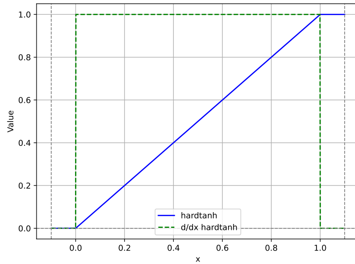
Fig. 9. The HardTanh function is shown in blue, and its derivative is represented by the green dashed line.
