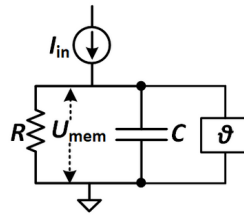
Fig. 2. RC model with switch: R represents the leakage resistance, I_{in} the input current, C the membrane capacitance, U_{mem} the membrane potential (i.e., the accumulated charge) and \vartheta a switch that lets the capacitor discharge (i.e. emit a spike) when a voltage threshold is reached. Source: [1]
