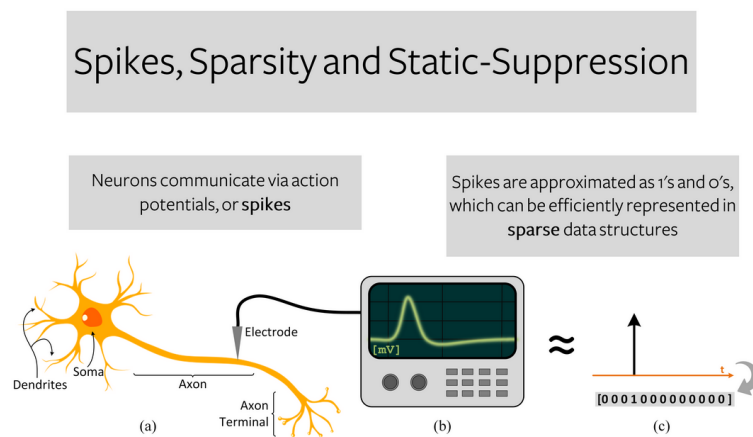
Fig. 3. Sparsity on Spike Neuron Networks. Source: [1]
