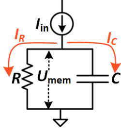
Fig. 5: RC model for currents: I_{in}(t) = I_R(t) + I_C(t)
