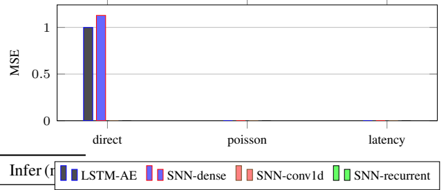
Figure 6. MSE comparison by model type and encoding. SNN modes trade reconstruction quality for reduced estimated energy.
