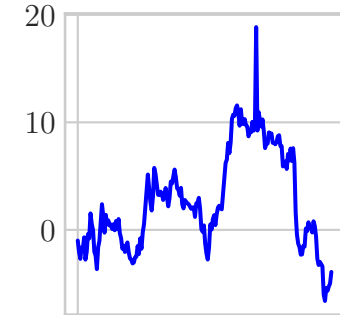
outlier
