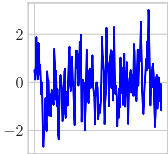
stationary
