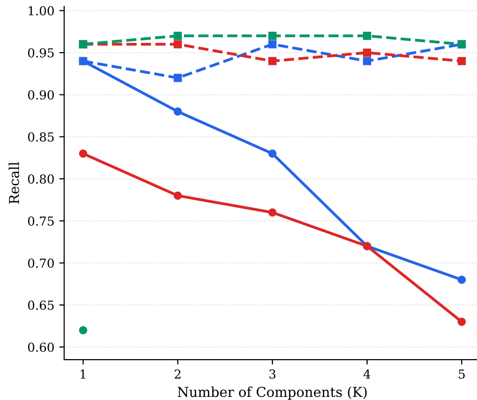
Recall
