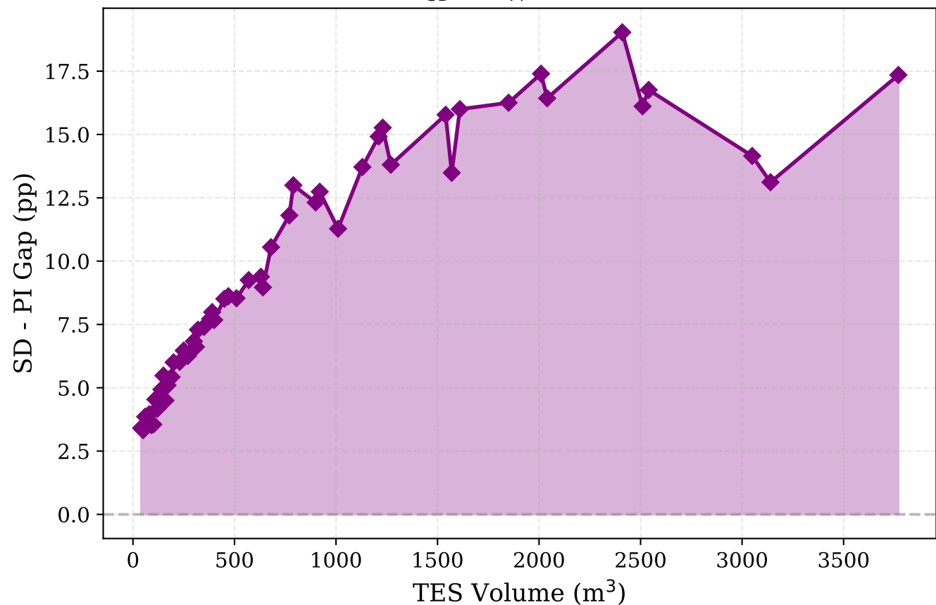
\Delta SF = SF_{SD} - SF_{PI} vs Tank Volume
