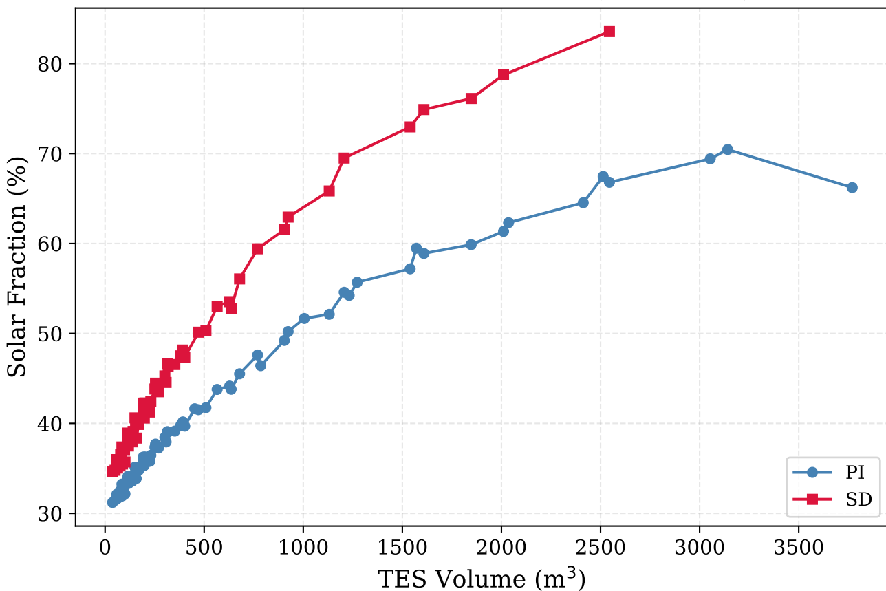
PI vs SD — SF vs Tank Volume (A=1000 m 2 )
