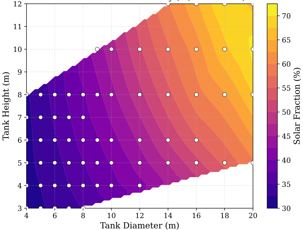
Solar Fraction vs Tank Geometry (PI, A=1000 \text{ m}^2 )
