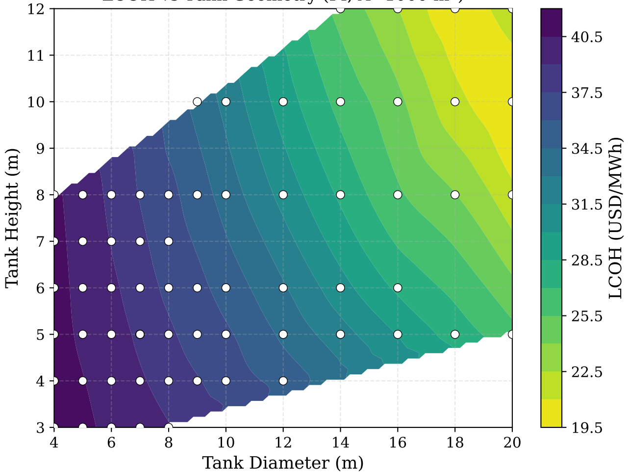
LCOH vs Tank Geometry (PI, A=1000 \text{ m}^2 )
