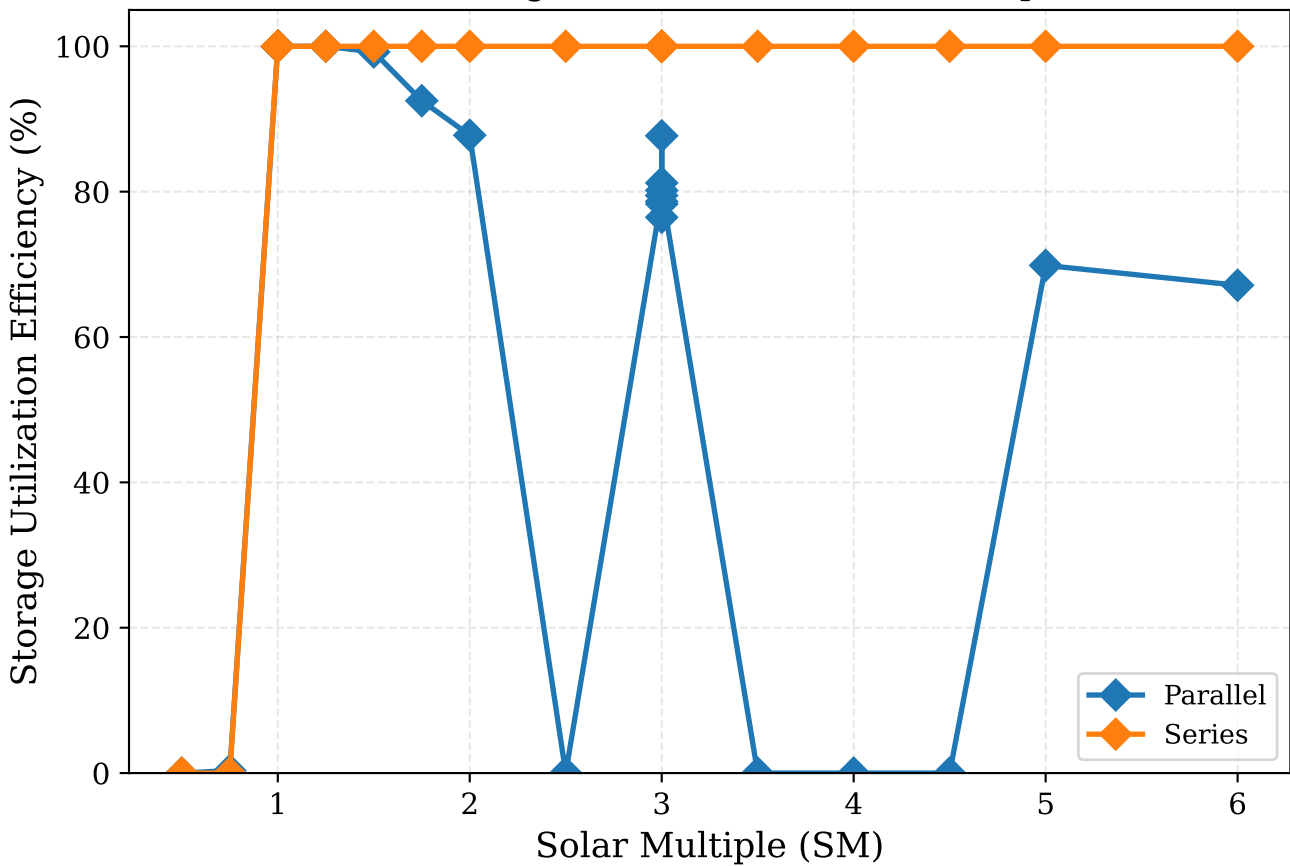
TES Storage Utilization vs Solar Multiple
